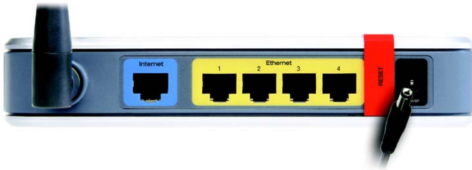
Figure 4-5: Connect the Power
