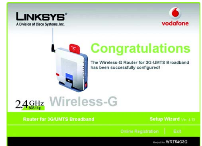
Figure 7-27: Congratulations Screen
