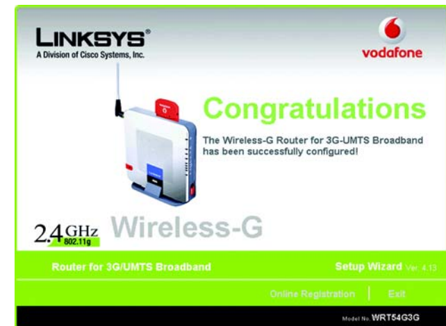
Figure 5-20: Congratulations Screen
