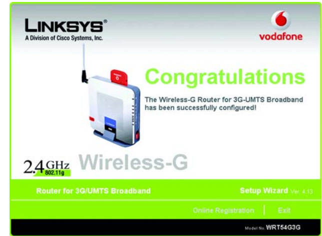
Figure 6-22: Congratulations Screen
